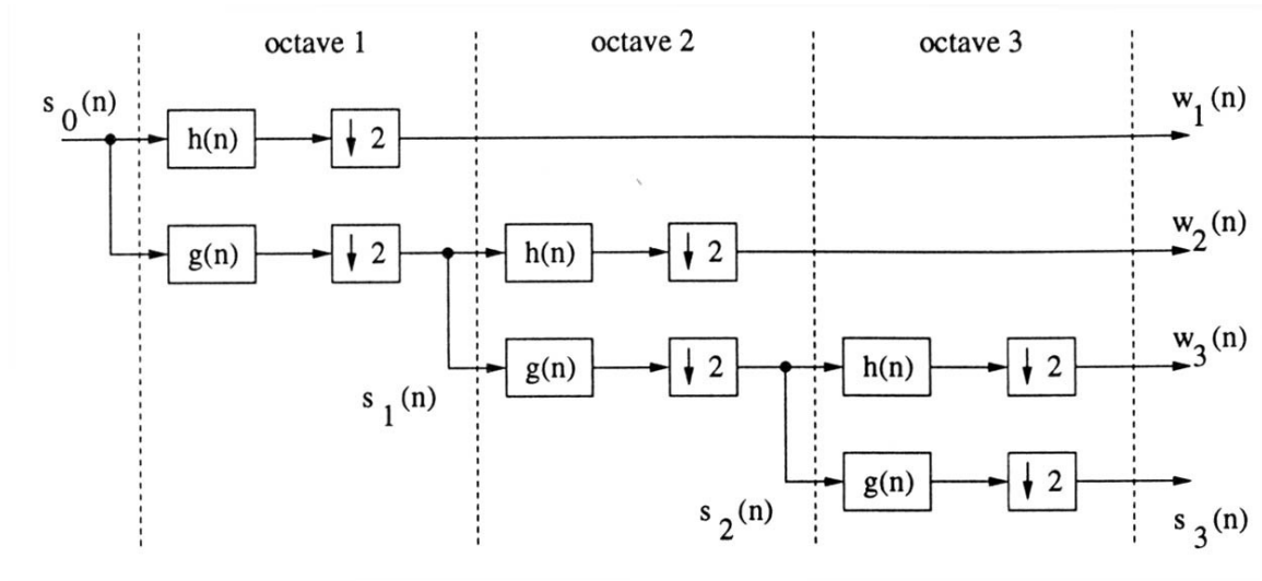
(a) One-dimensional 3-level DWT transform
